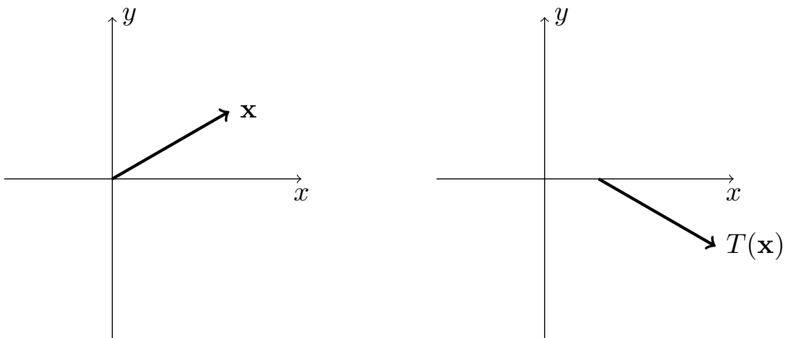
Figure 12.12 Glide reflections
