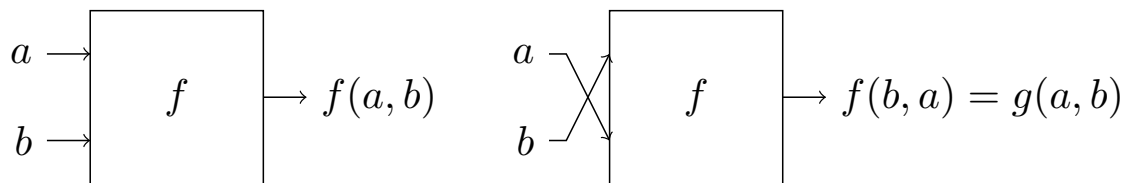
Figure 14.25 A switching function of two variables
